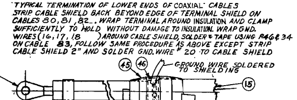
Figure 13—Center Panel Connections (TT-618412)
