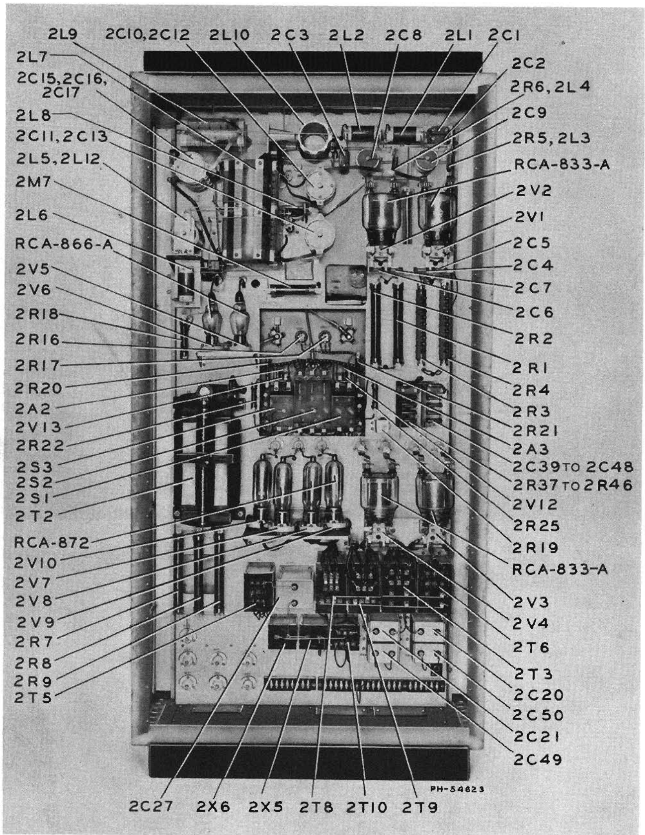
Figure 8—Amplifier-Modulator Chassis (Rear View)
